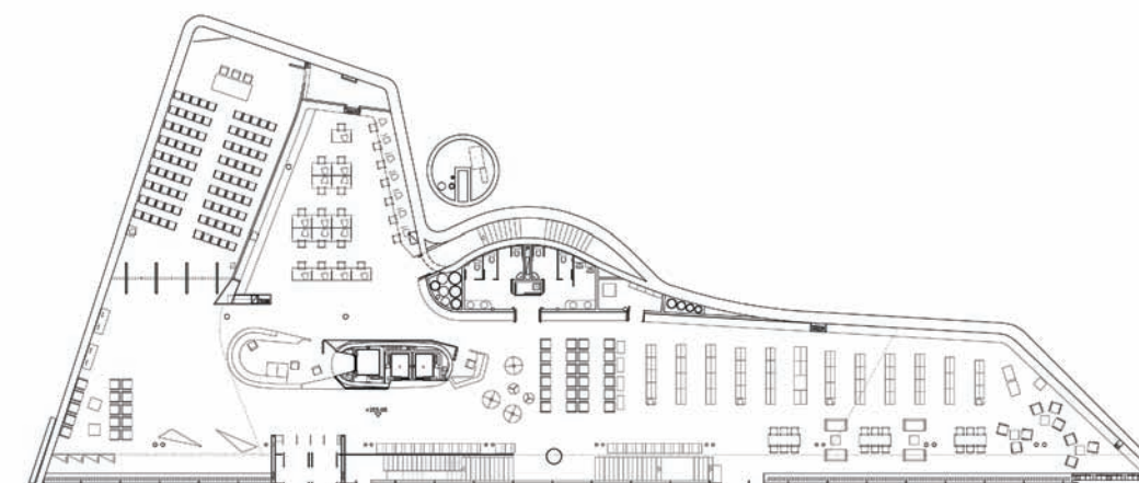
PLANTA BAJA / GROUND FLOOR PLAN
